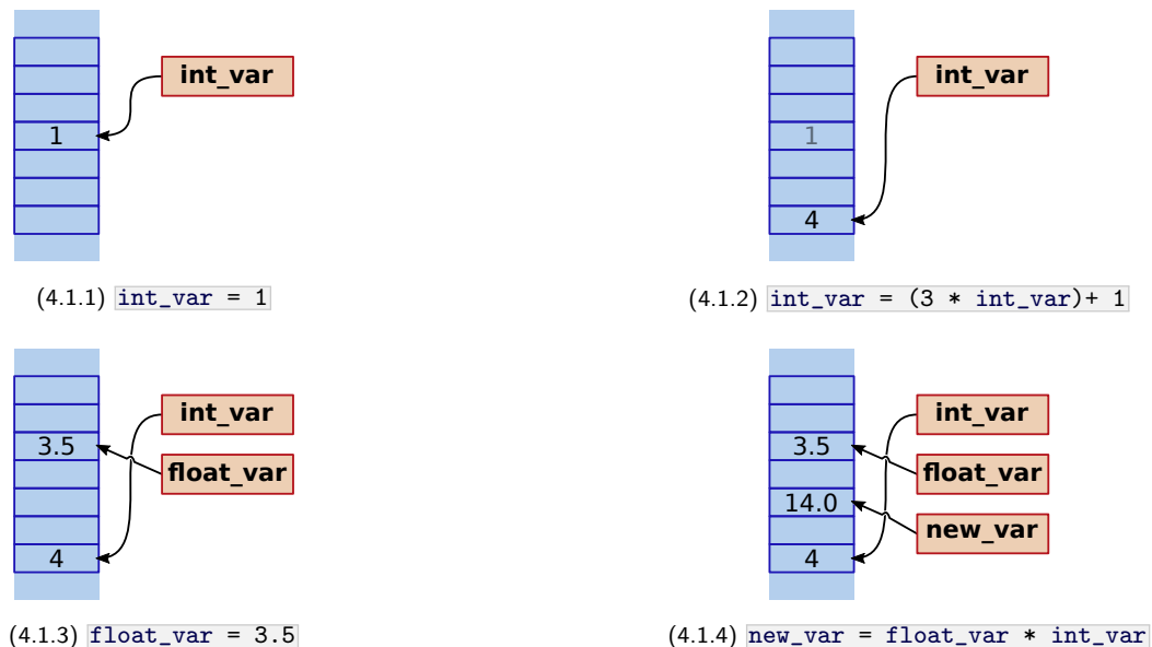
Figure 4.1: Illustrations of the variable assignments in Listing 4.1 in the same order in which they appear in the program: Variables are basically names that point to objects which are located somewhere in memory.
